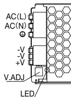
PS3V-030AF
