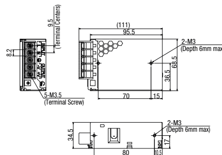
PS3V-030AF □ C
