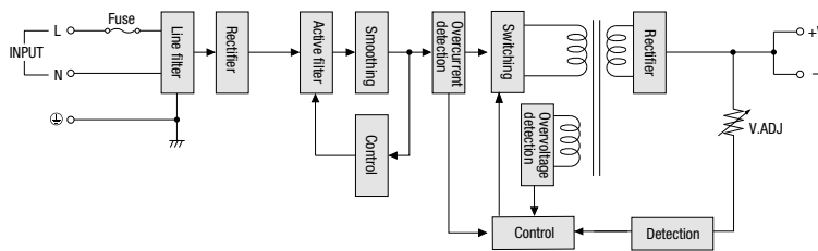
PS3V-100AF, PS3V-150AF
