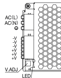
PS3V-100AF
