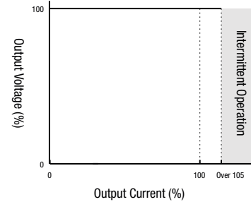
PS3V-100AF / -150AF
