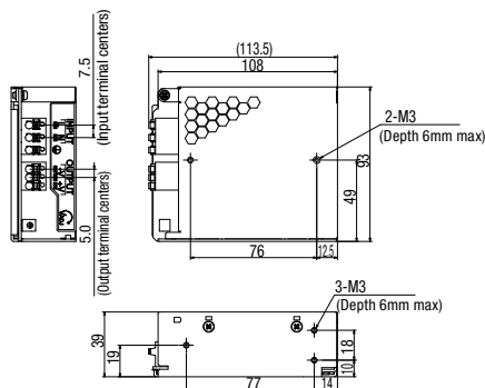
PS3V-100AF24P
