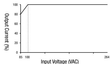
PS3V-100AF / -150AF
