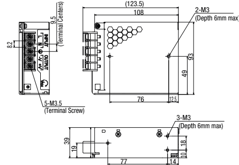
PS3V-100AF24C
