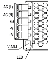
PS3V-030AF
