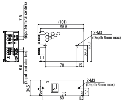
PS3V-100AF24P
