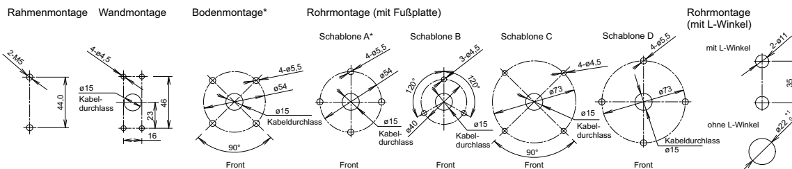
Abmessungen in mm.
