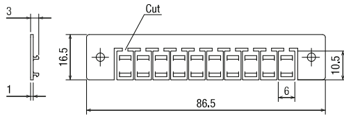
Marking Plate SV9Z-PW10
