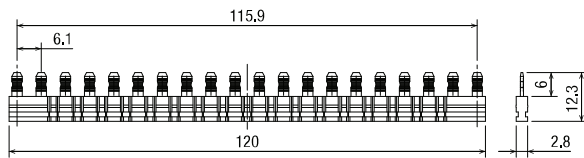
Jumper SV9Z-J20*PN10
