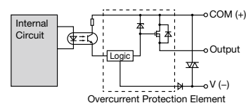
FC6A-T08P1/FC6A-T16P1 FC6A-T16P3/FC6A-T32P3
