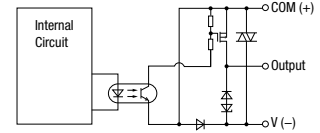
FC6A-PTS4
