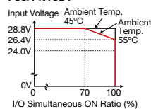
FC6A-N08A11
