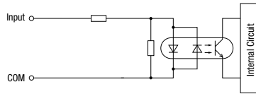
FC6A-PN4
