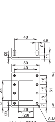
IAC-L5 (for IAC-R8)
