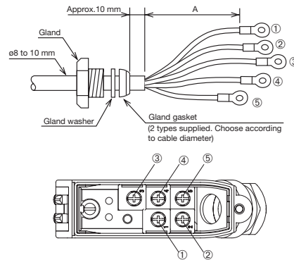
Recommended insulation length (A)
