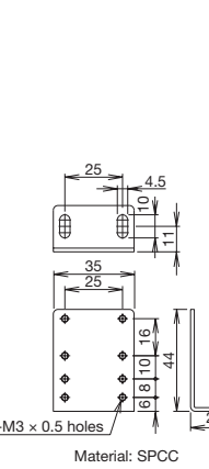
IAC-L3 (for IAC-R6)
