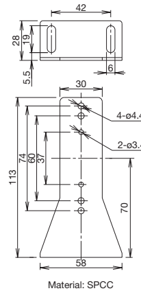
IAC-L2 (for IAC-R5)
