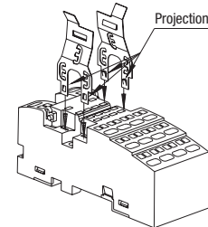
SFA-202 Leaf Spring
