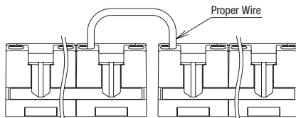
Jumper Wiring of Terminal 14 between Adjoining Sockets
